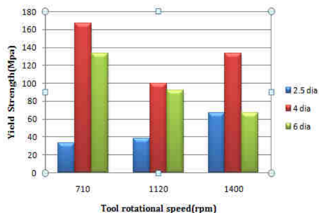
Graph.1: Effect of tool pin diameters and rotational speed on yield strength
