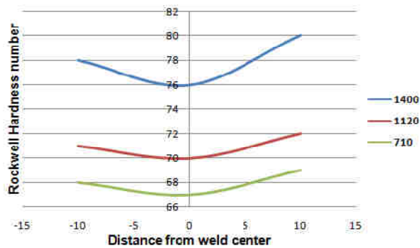
Graph.4: Effect of 2.5mm pin and rotational speed on hardness
