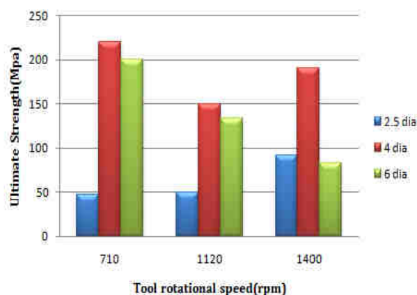
Graph.2: Effect of tool pin diameters and rotational speed on ultimate strength
