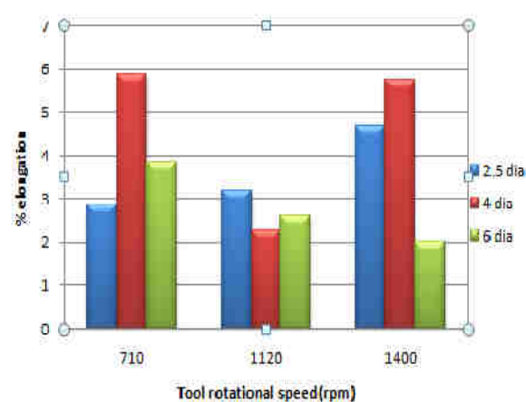
Graph.3: Effect of tool pin diameters and rotational speed on percent of elongation
